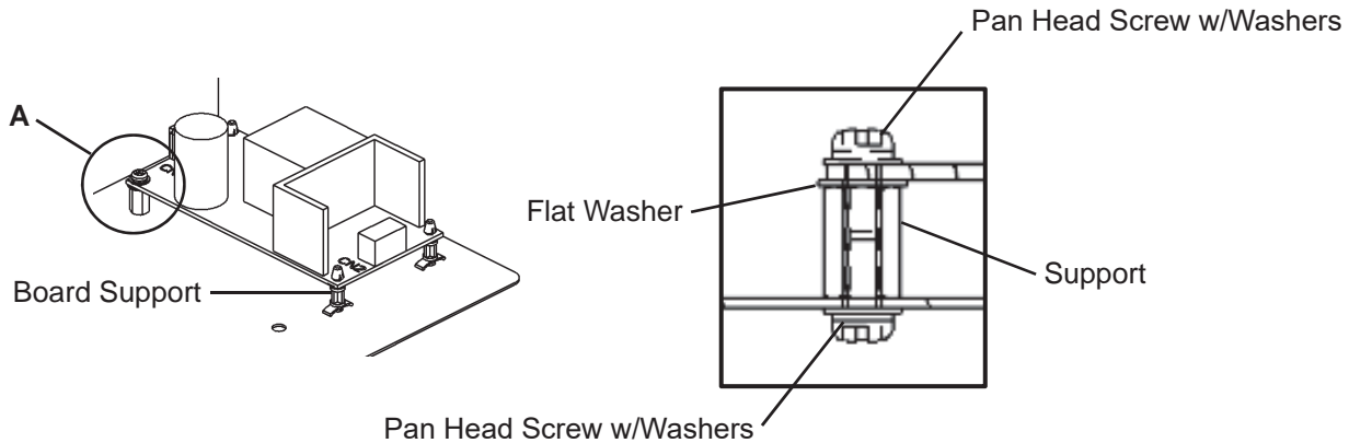
Detail A
