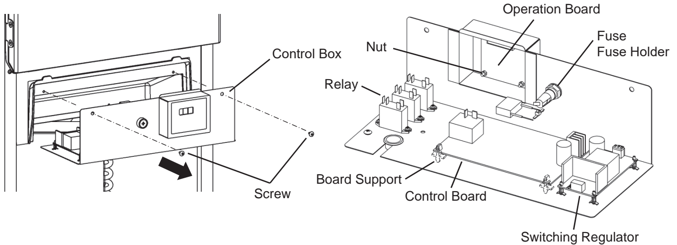
Control Box
